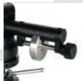
Any weight of cartridge can be accommodated by virtue of the easily interchangeable counterweights
